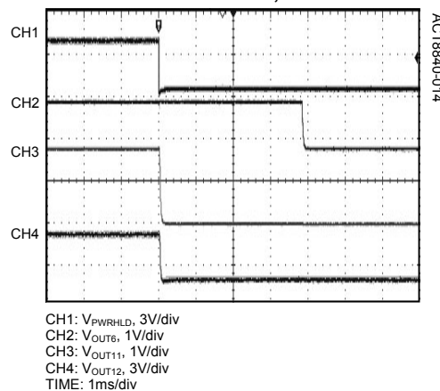
Shutdown of PWRHLD, OUT6/11/12
