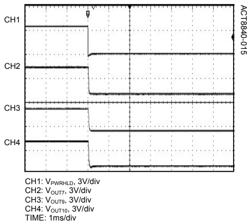
Shutdown of PWRHLD, OUT7/9/10
