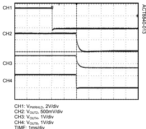
Shutdown of PWRHLD, OUT2/4/8
